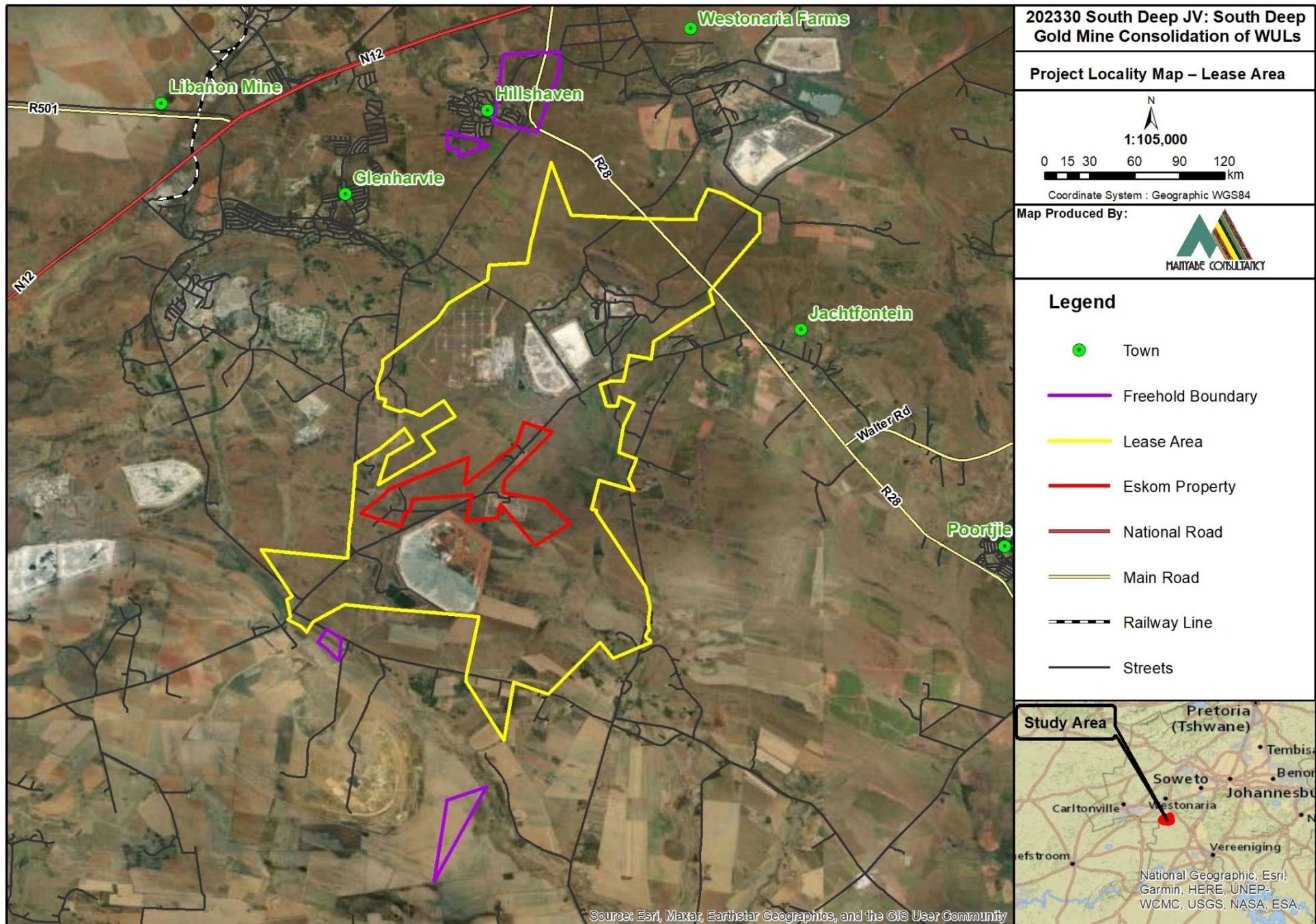
Figure 1: Locality Map
