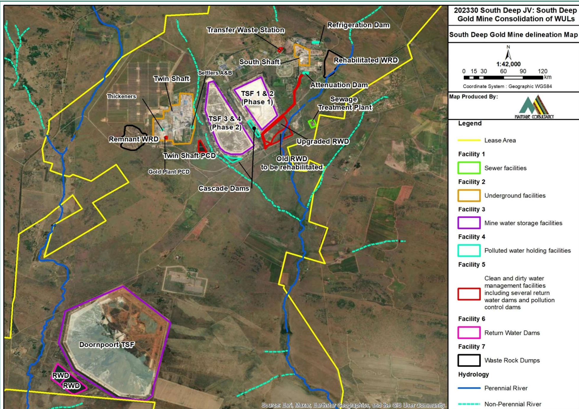
Figure 2: Mine Layout Plan
